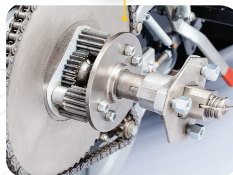
Patented QuickLock Differential (Deluxe Model)
